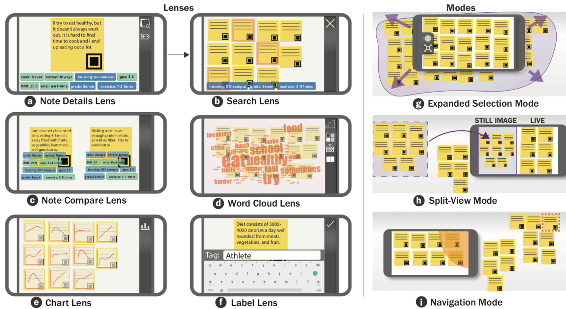
Figure 4: A sampling of Affinity Lens AR Lenses.
